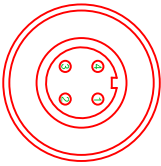
WIRE ENTRY HR10A-7P-4P(73)
